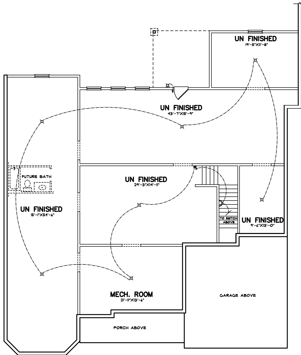
BASEMENT PLAN
