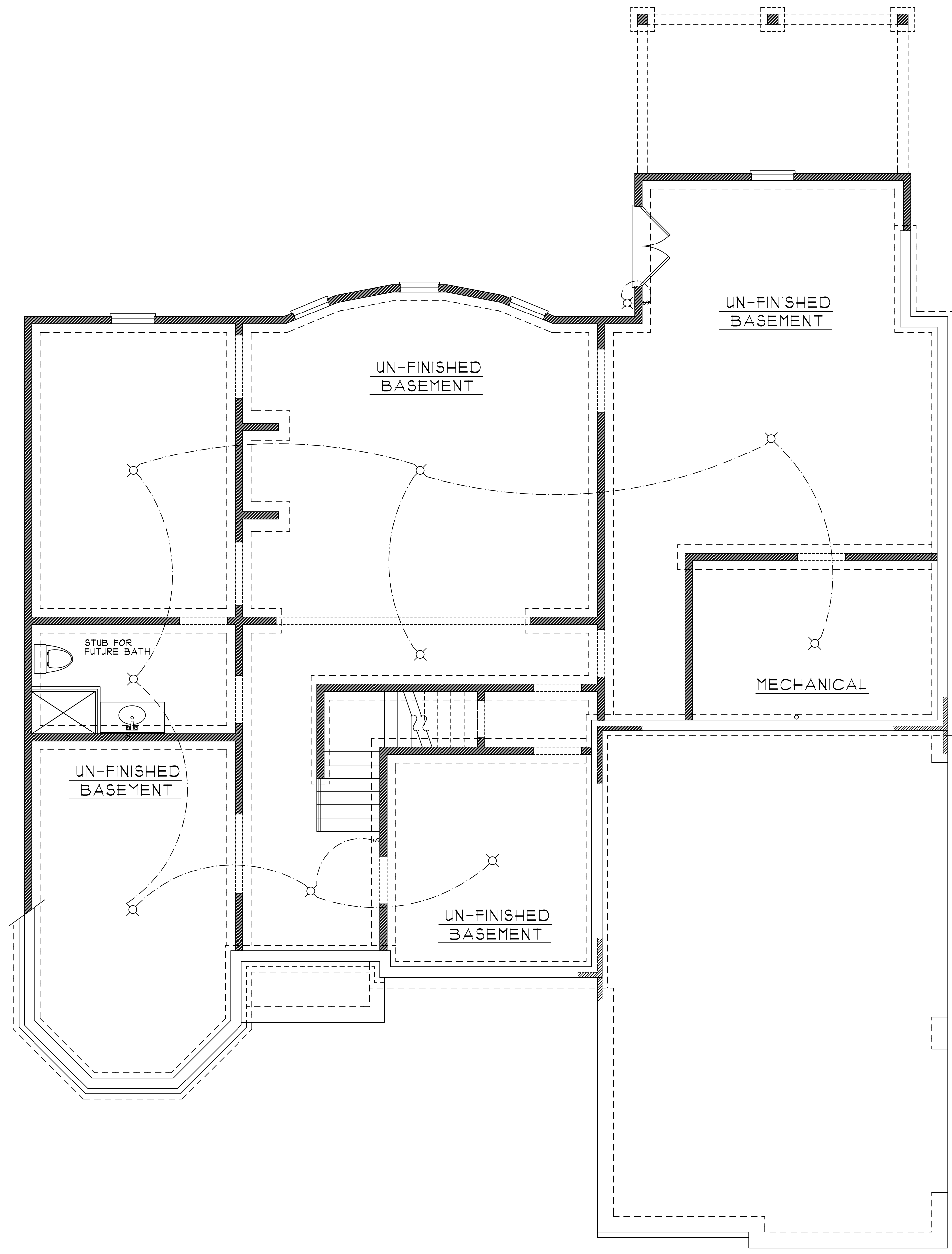
BASEMENT FLOOR PLAN
