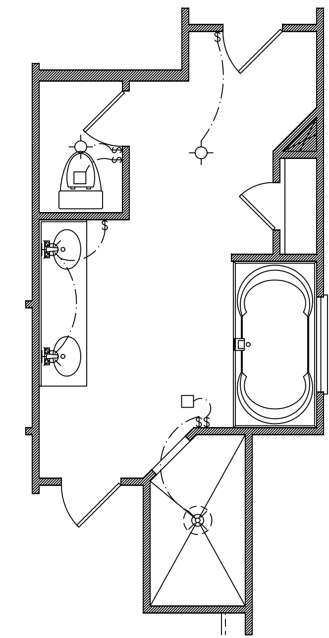
MASTER BATH OPTION
