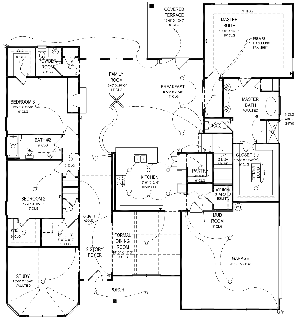
FIRST FLOOR
