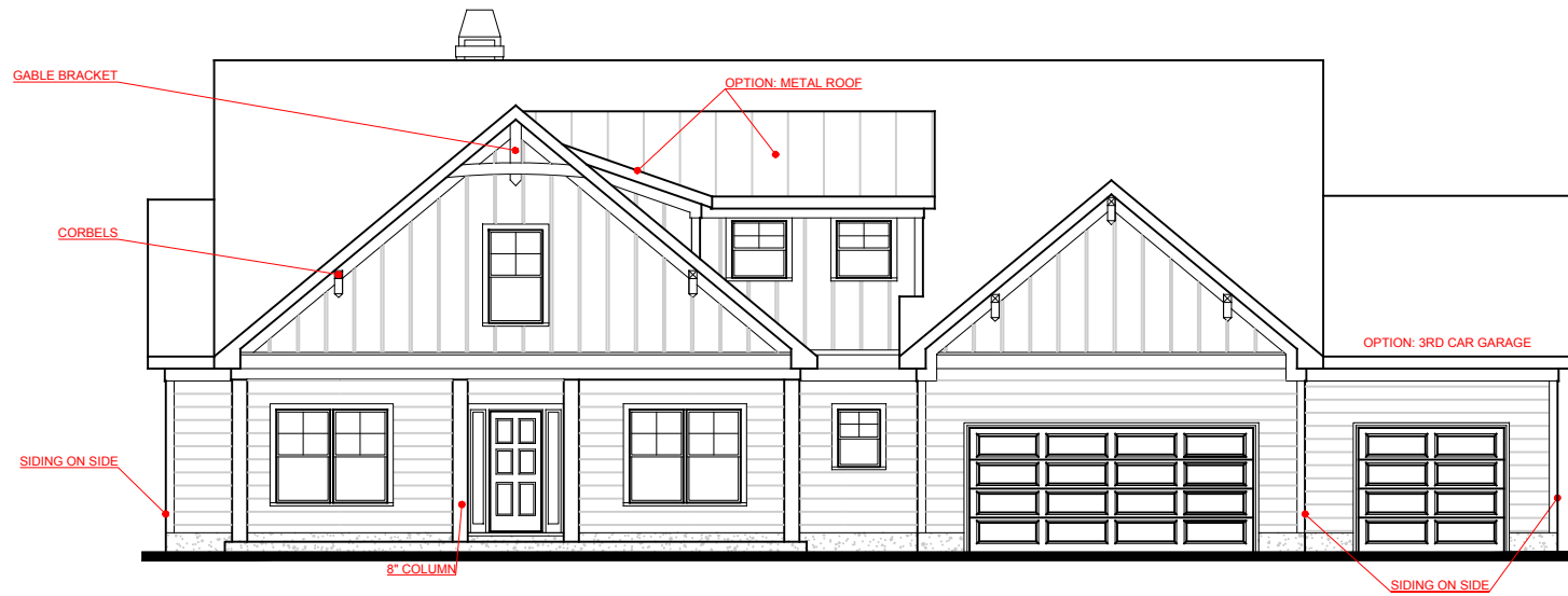
FRONT ELEVATION- A VERSION
