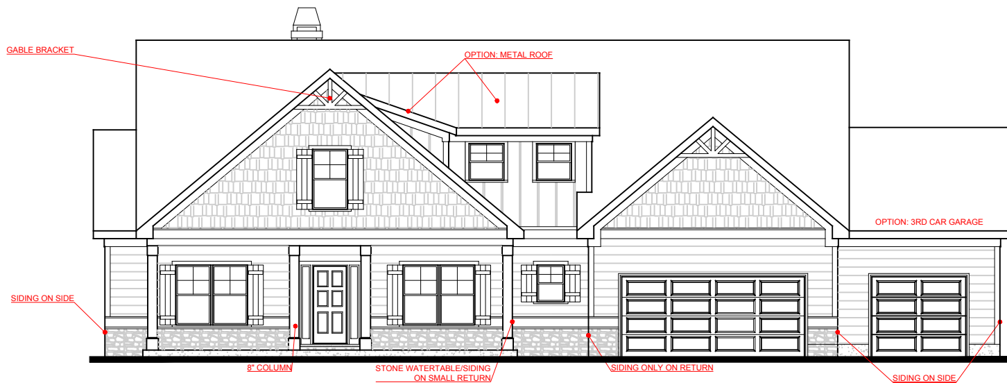
FRONT ELEVATION- B VERSION
