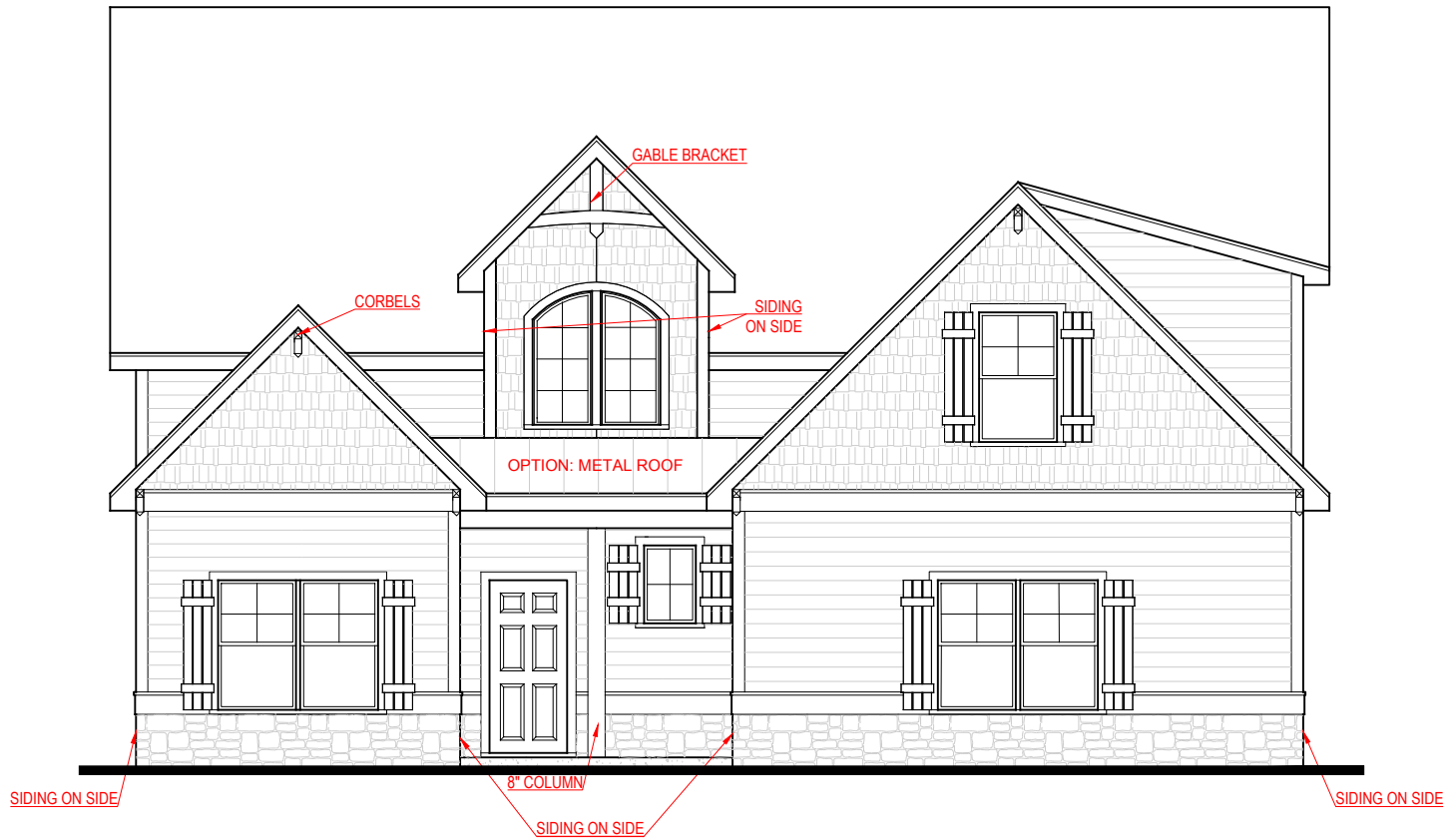
FRONT ELEVATION - B VERSION
