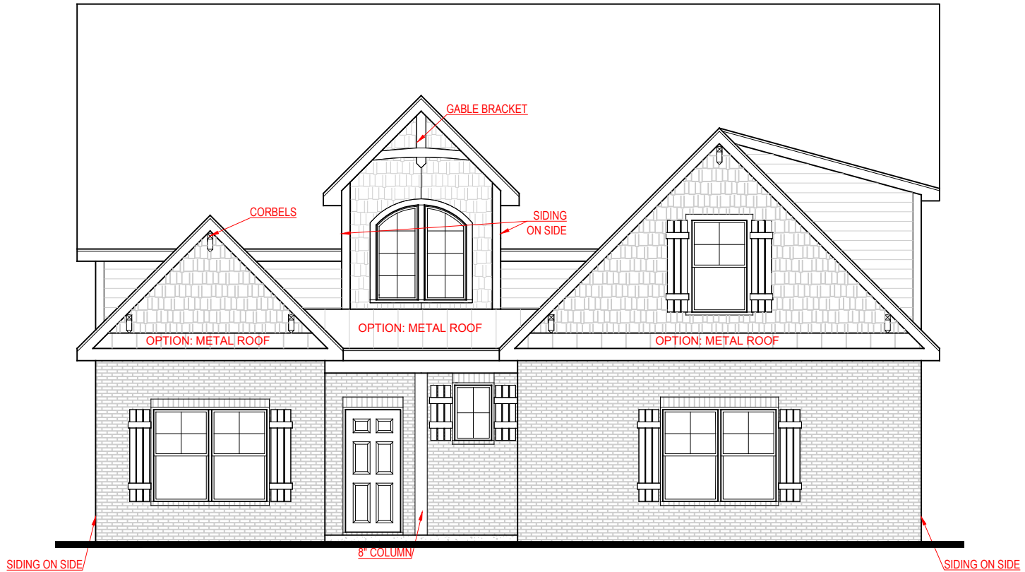
FRONT ELEVATION - D VERSION
