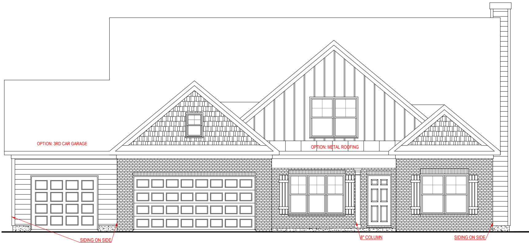
FRONT ELEVATION - B-D VERSION
