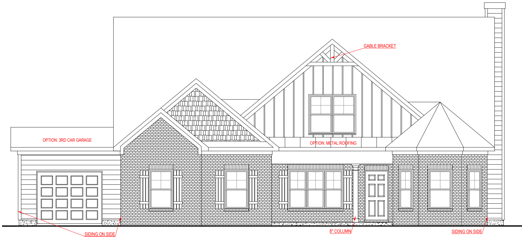
FRONT ELEVATION - C-D VERSION
