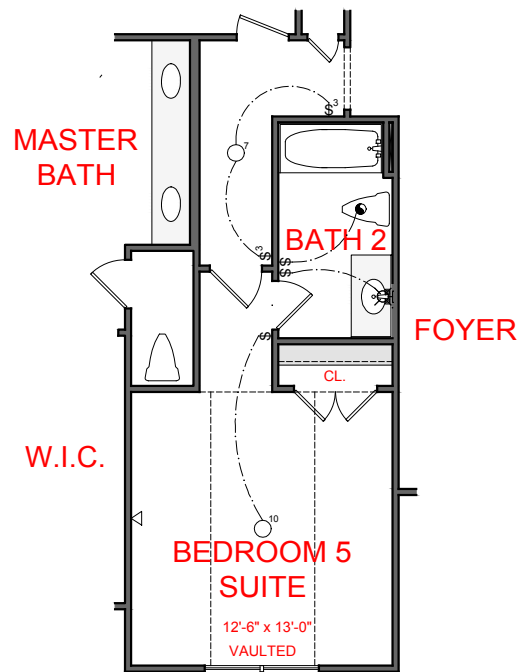
OPTION: BEDROOM 5 SUITE
