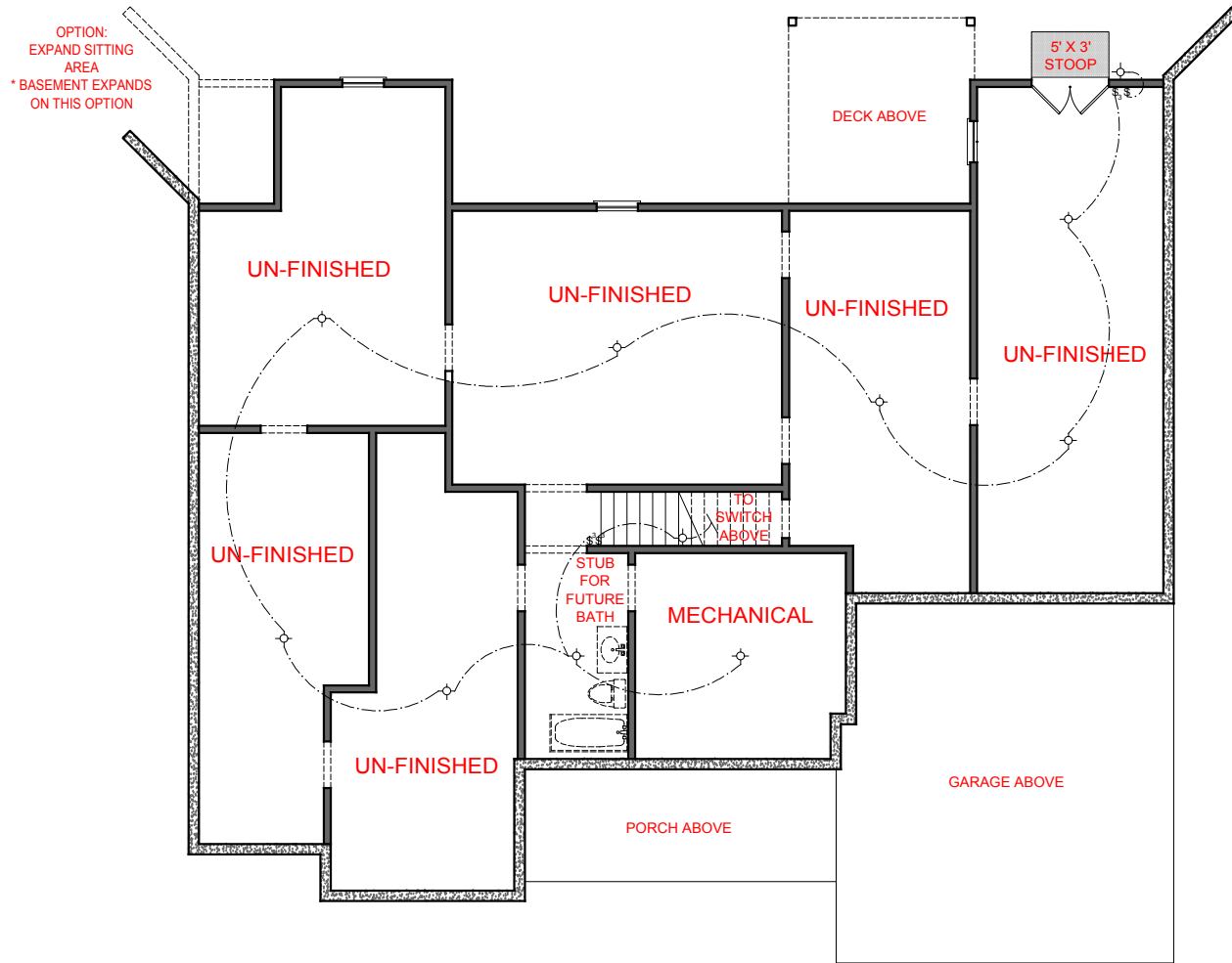
OPTION: BASEMENT PLAN
