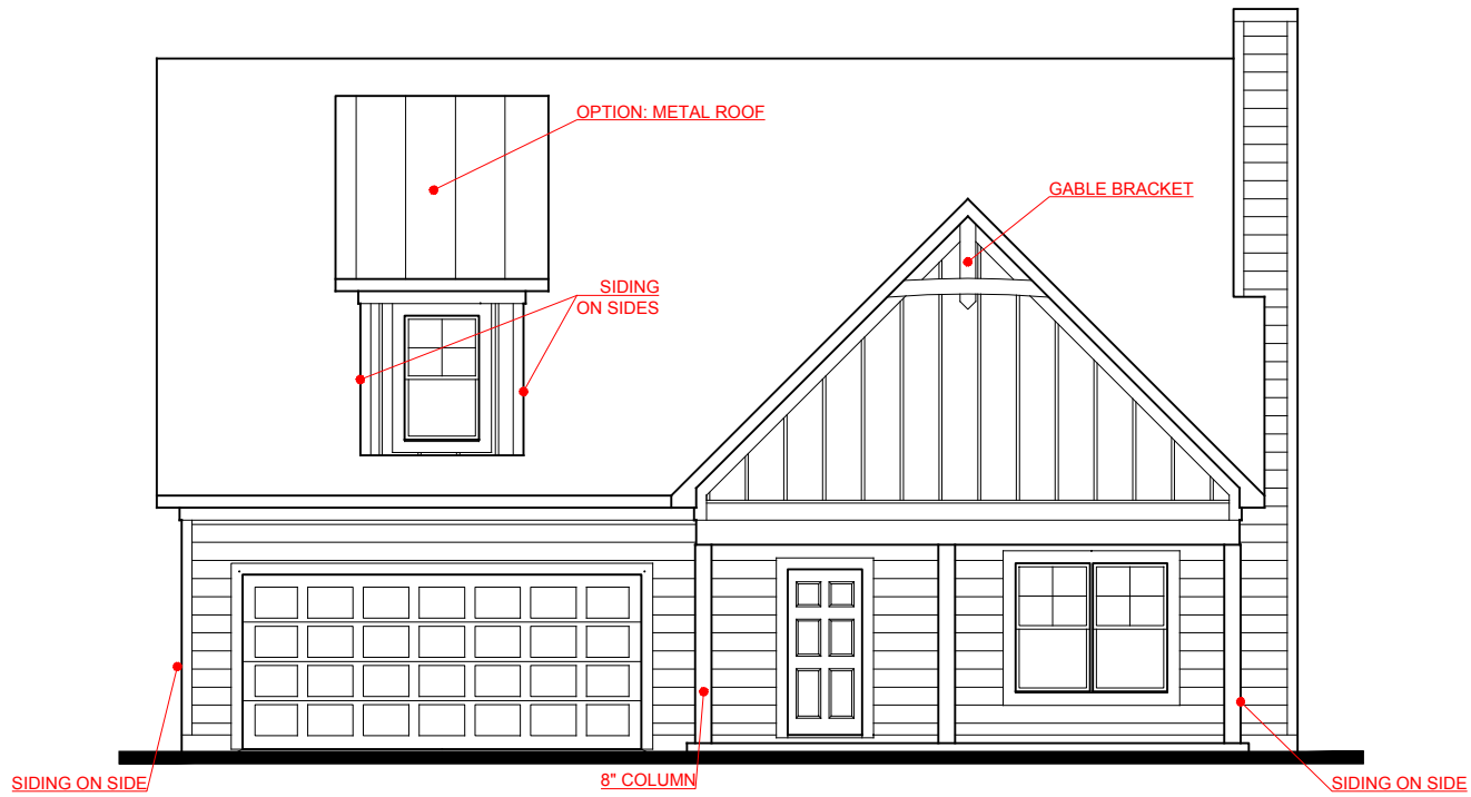
FRONT ELEVATION- A VERSION
