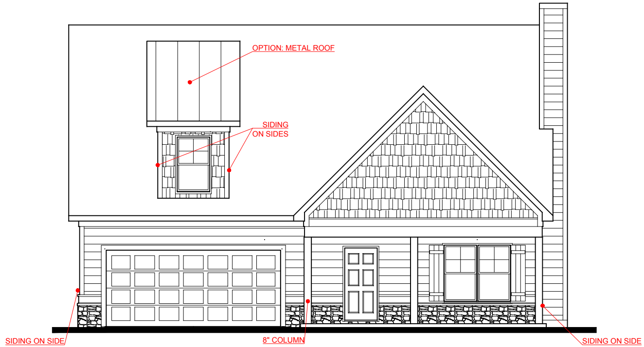
FRONT ELEVATION- B VERSION
