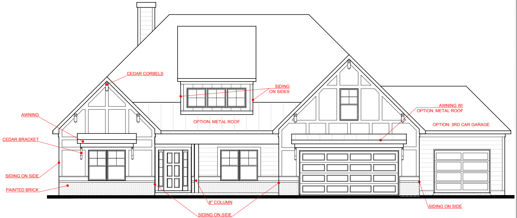
FRONT ELEVATION- F VERSION
