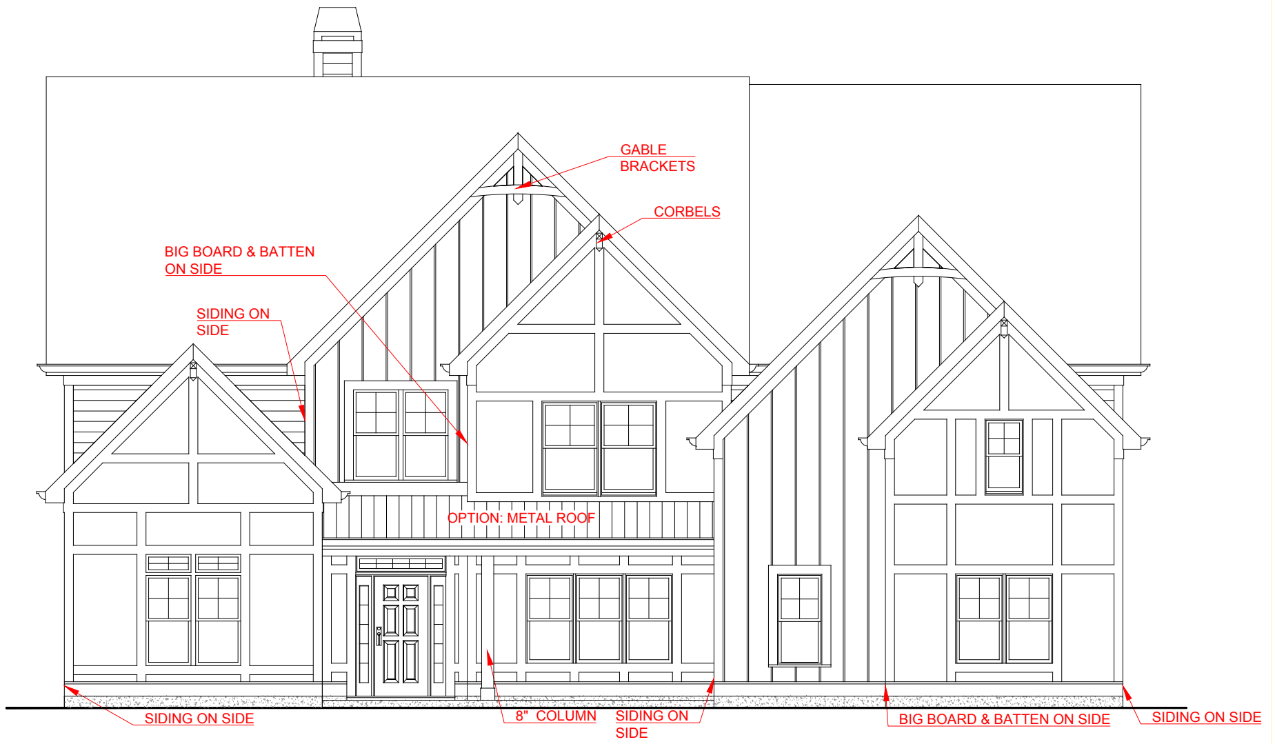
FRONT ELEVATION - A VERSION
