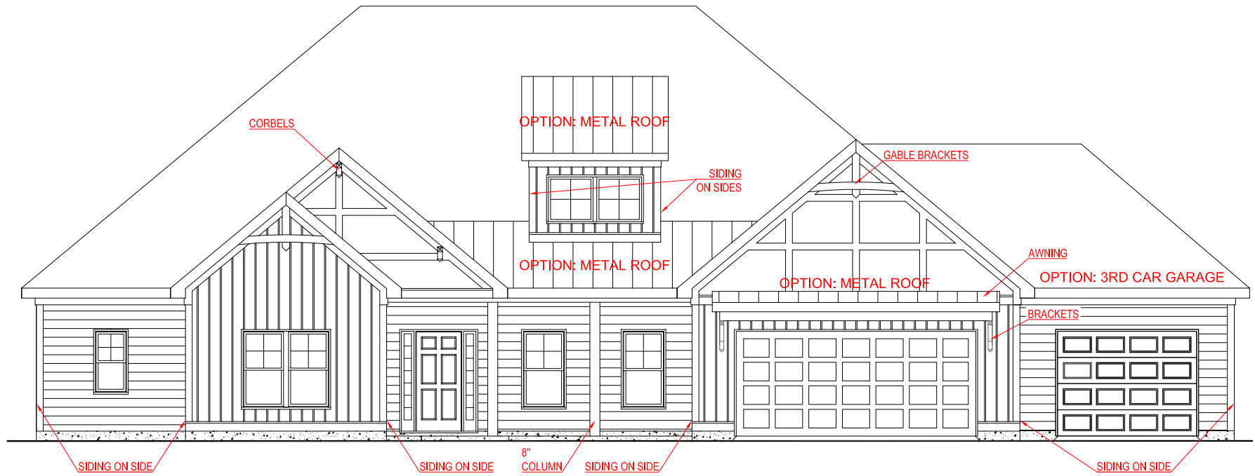
FRONT ELEVATION - A VERSION
