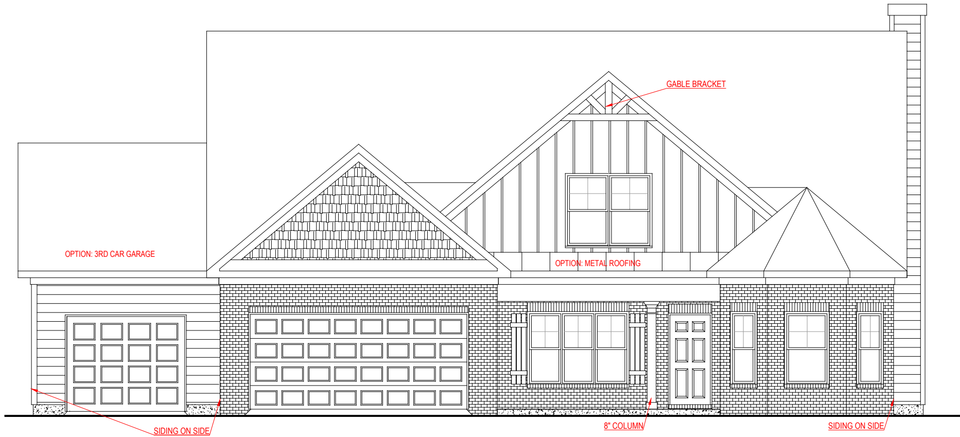
FRONT ELEVATION - C-D VERSION
