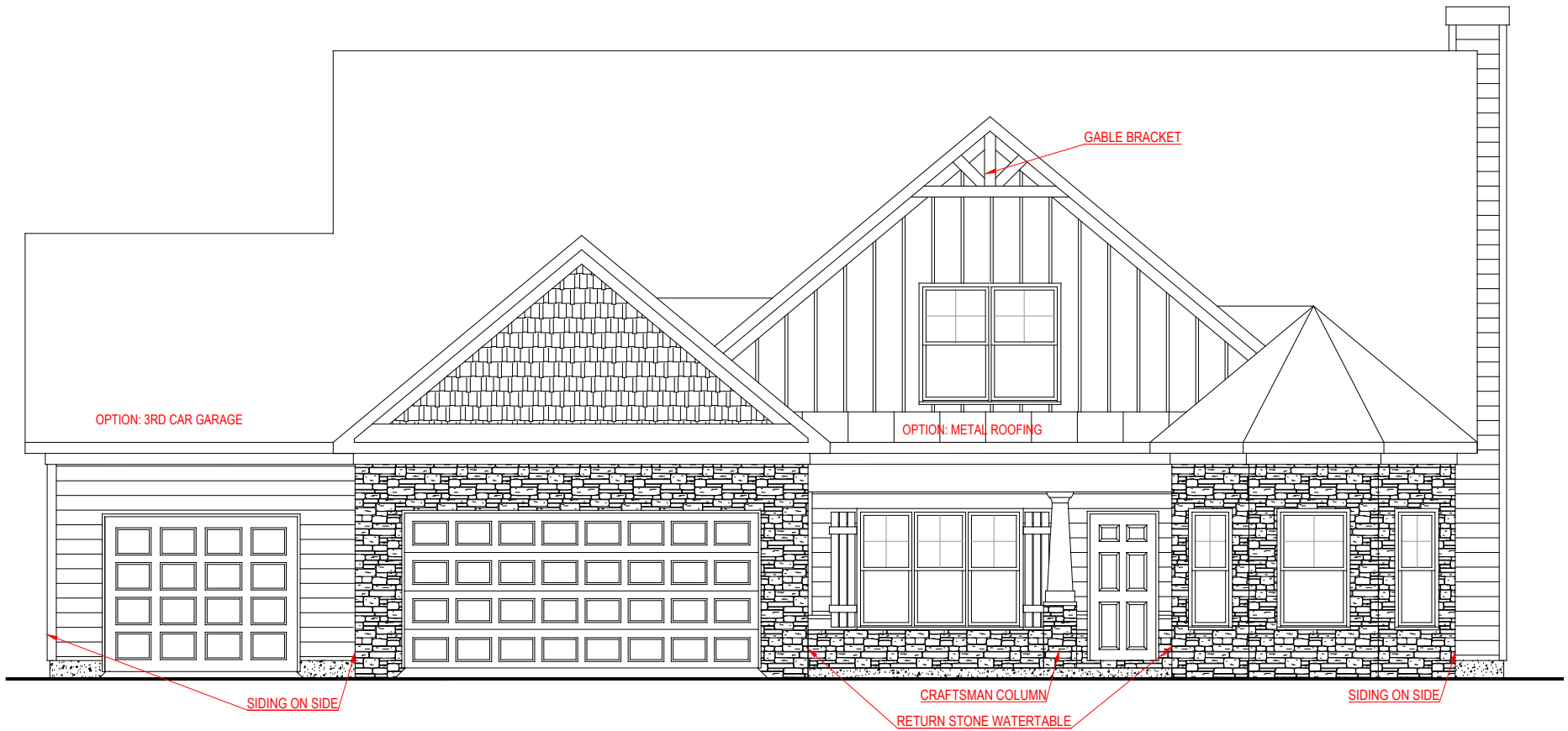
FRONT ELEVATION - C VERSION
