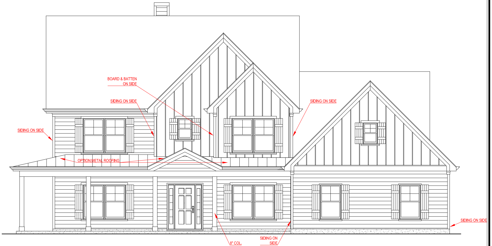
FRONT ELEVATION - A VERSION
