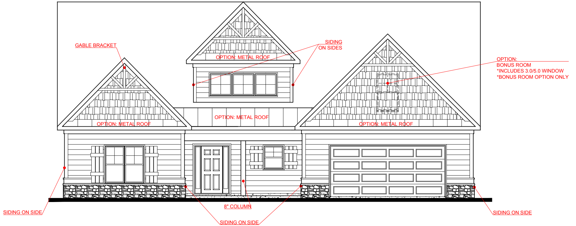
FRONT ELEVATION- B VERSION
