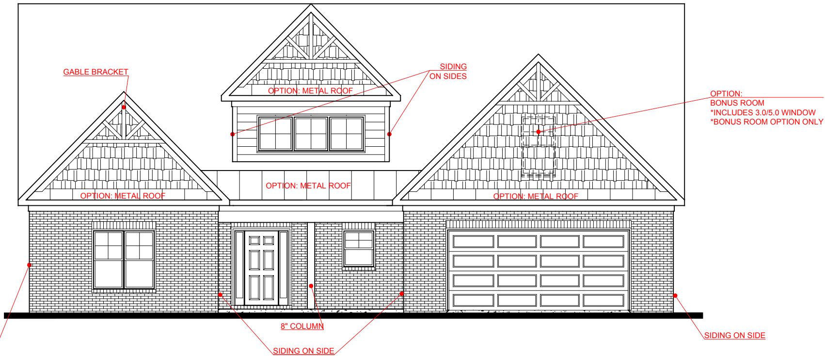
FRONT ELEVATION- D VERSION
