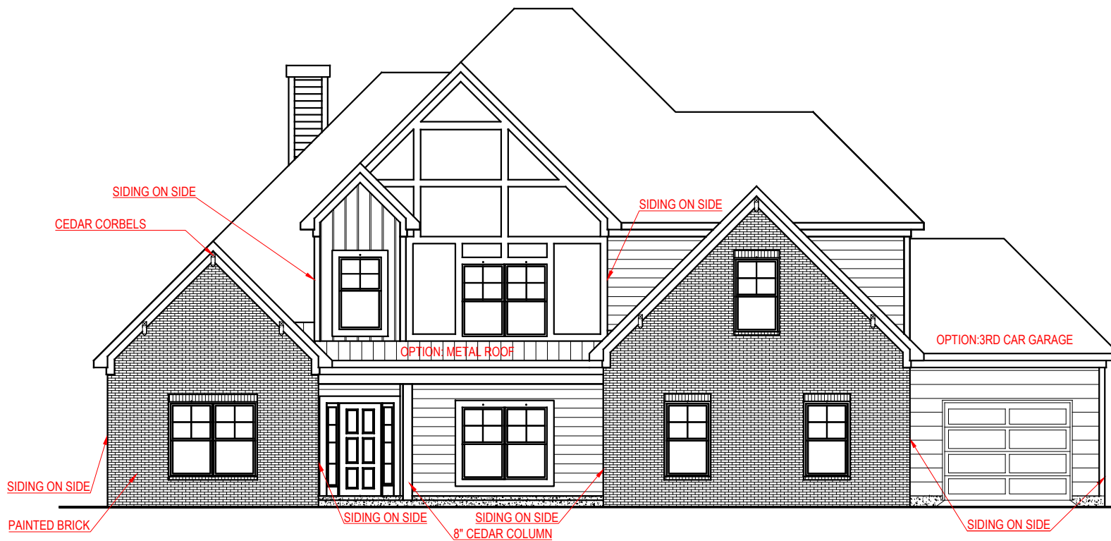
FRONT ELEVATION - F VERSION
