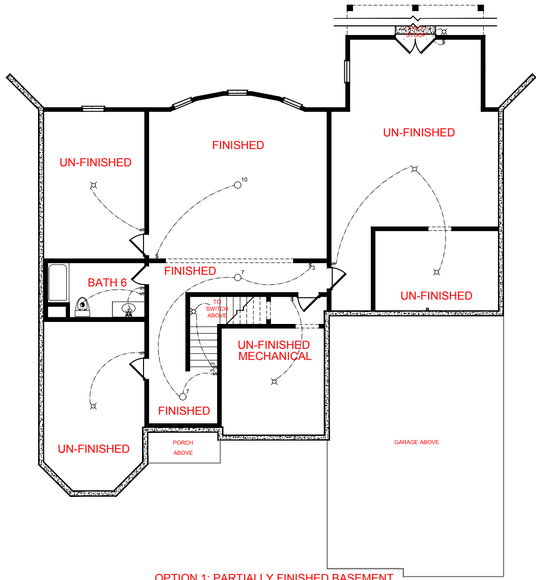
OPTION 1: PARTIALLY FINISHED BASEMENT *ADD 641 SQ. FT.
