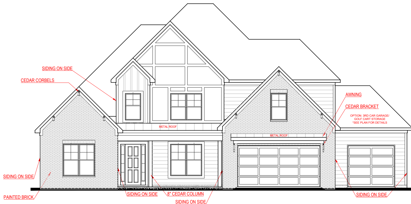
FRONT ELEVATION - F VERSION
