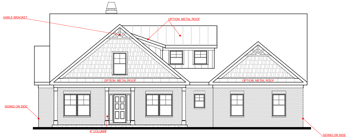
FRONT ELEVATION- D VERSION
