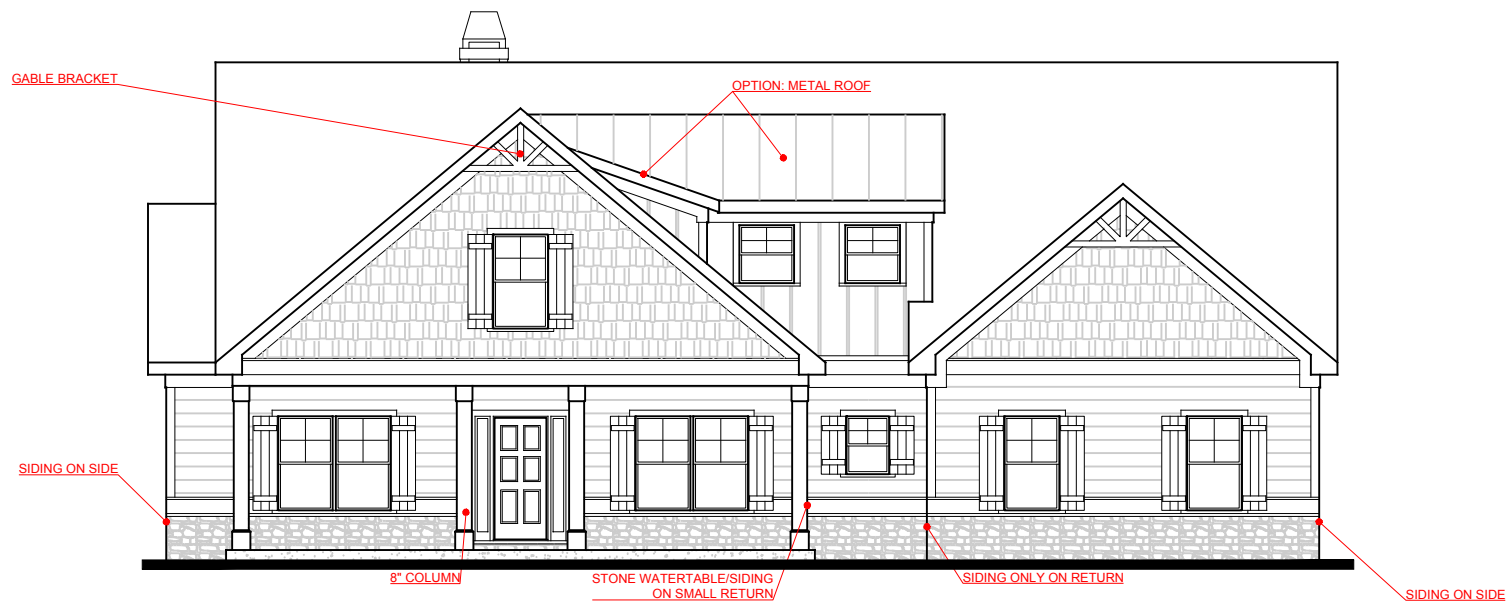
FRONT ELEVATION- B VERSION
