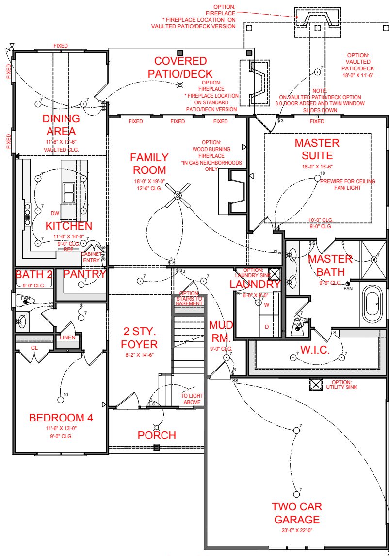
FIRST FLOOR PLAN * NO 1ST FLOOR
