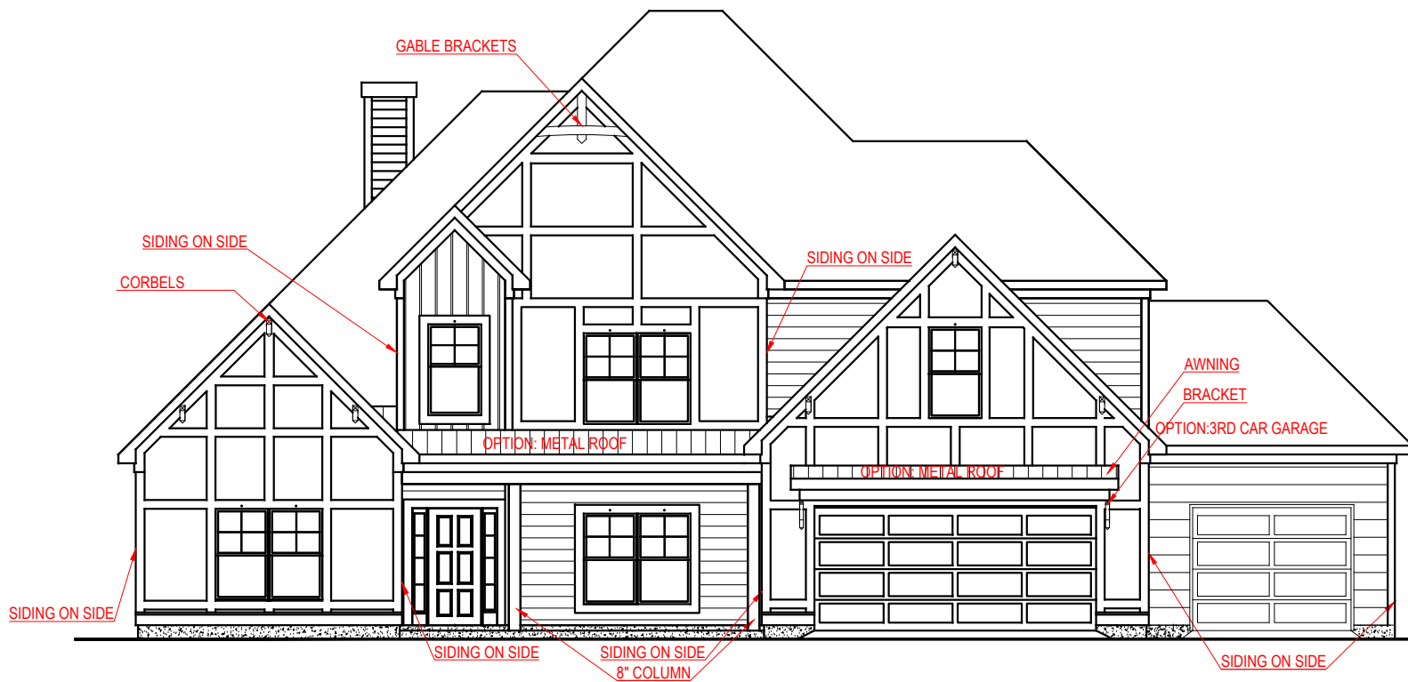
FRONT ELEVATION - A VERSION
