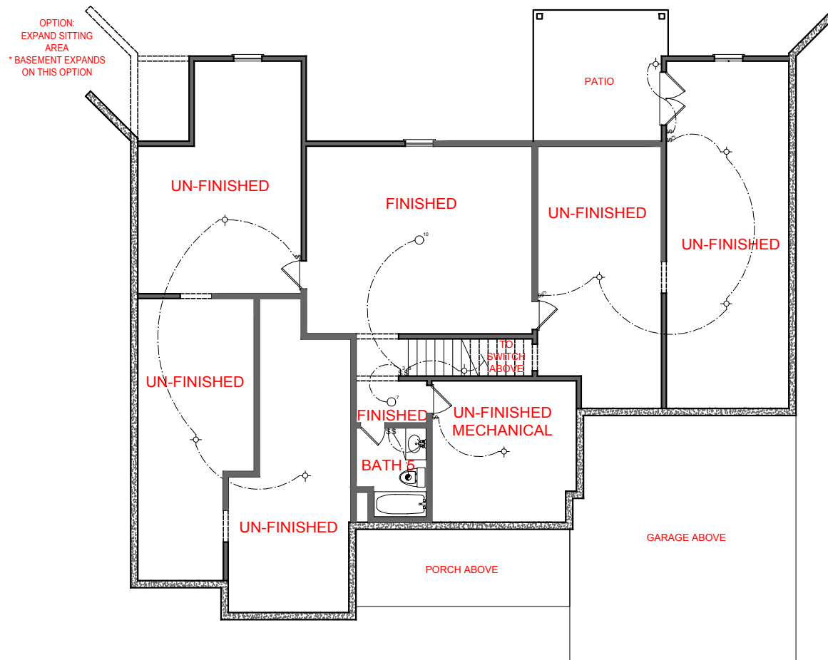
OPTION TWO: PARTIALLY FINISHED BASEMENT PLAN 529 SQ. FT. FINISHED
