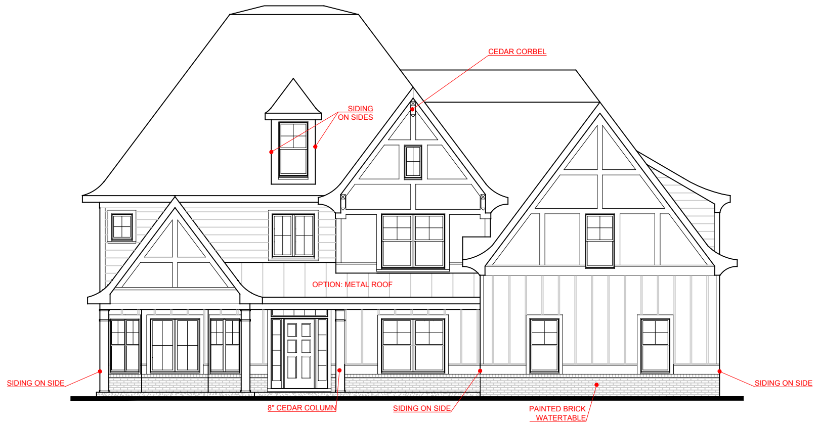
FRONT ELEVATION- F VERSION
