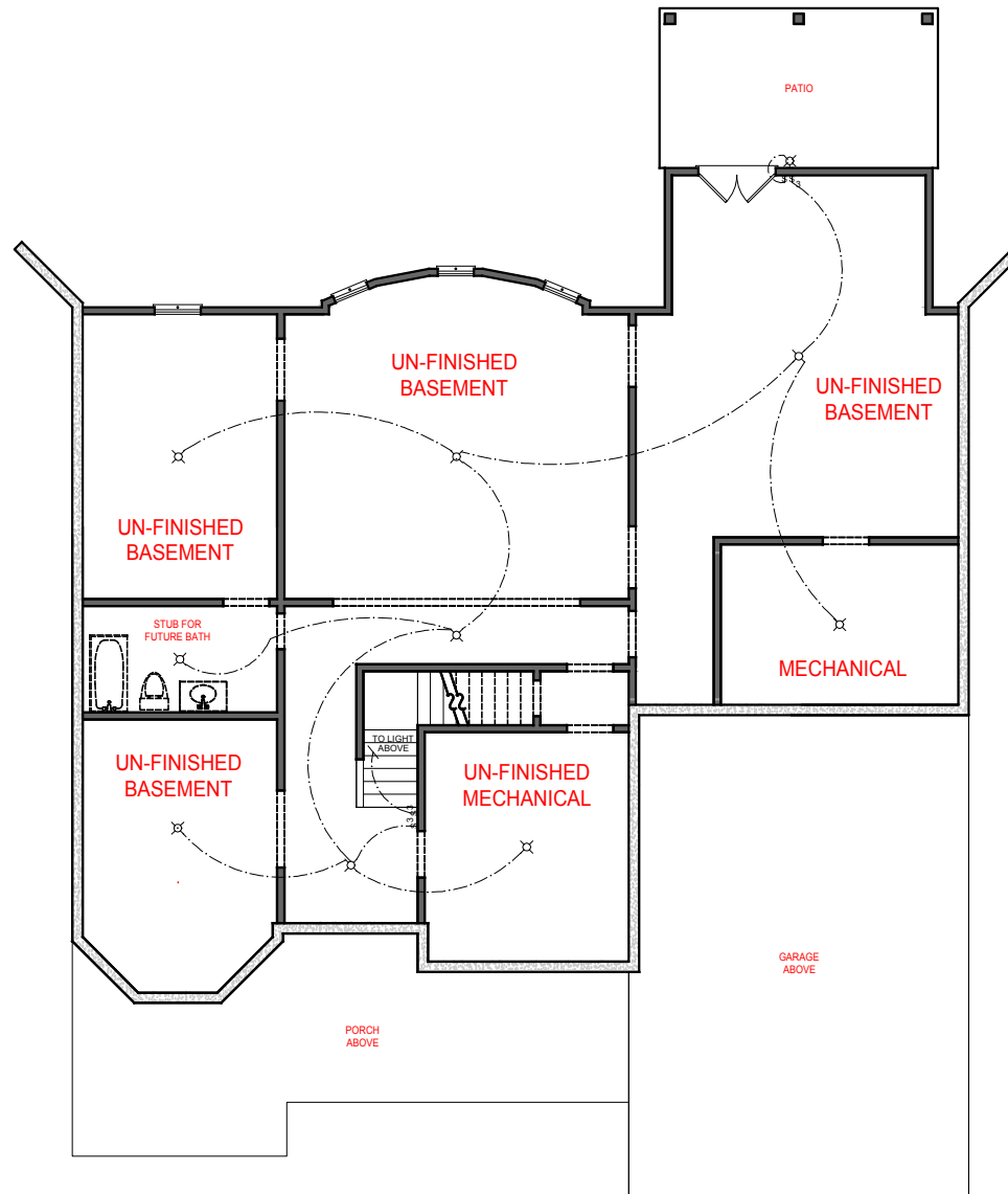
OPTION 1: UN-FINISHED BASEMENT PLAN
