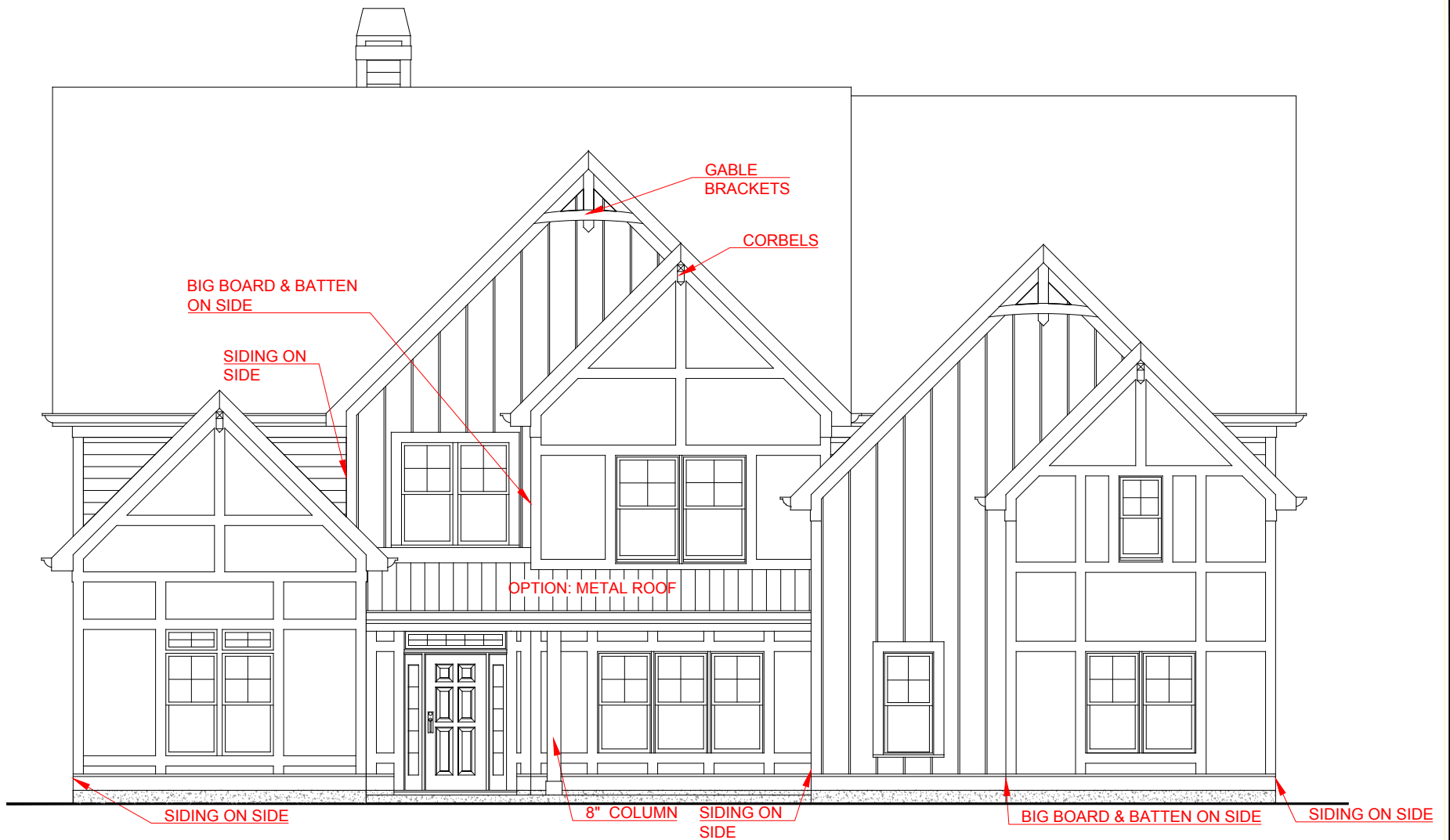
FRONT ELEVATION - A VERSION
