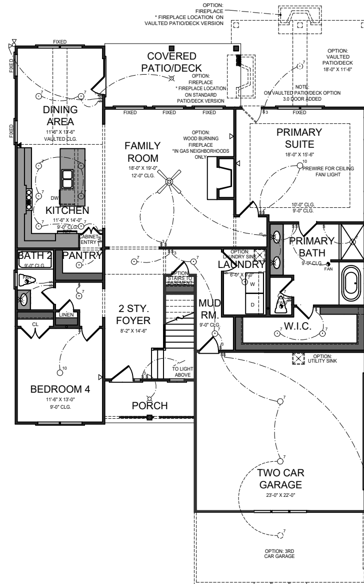
FIRST FLOOR PLAN NOT TO FIRST FLOOR
