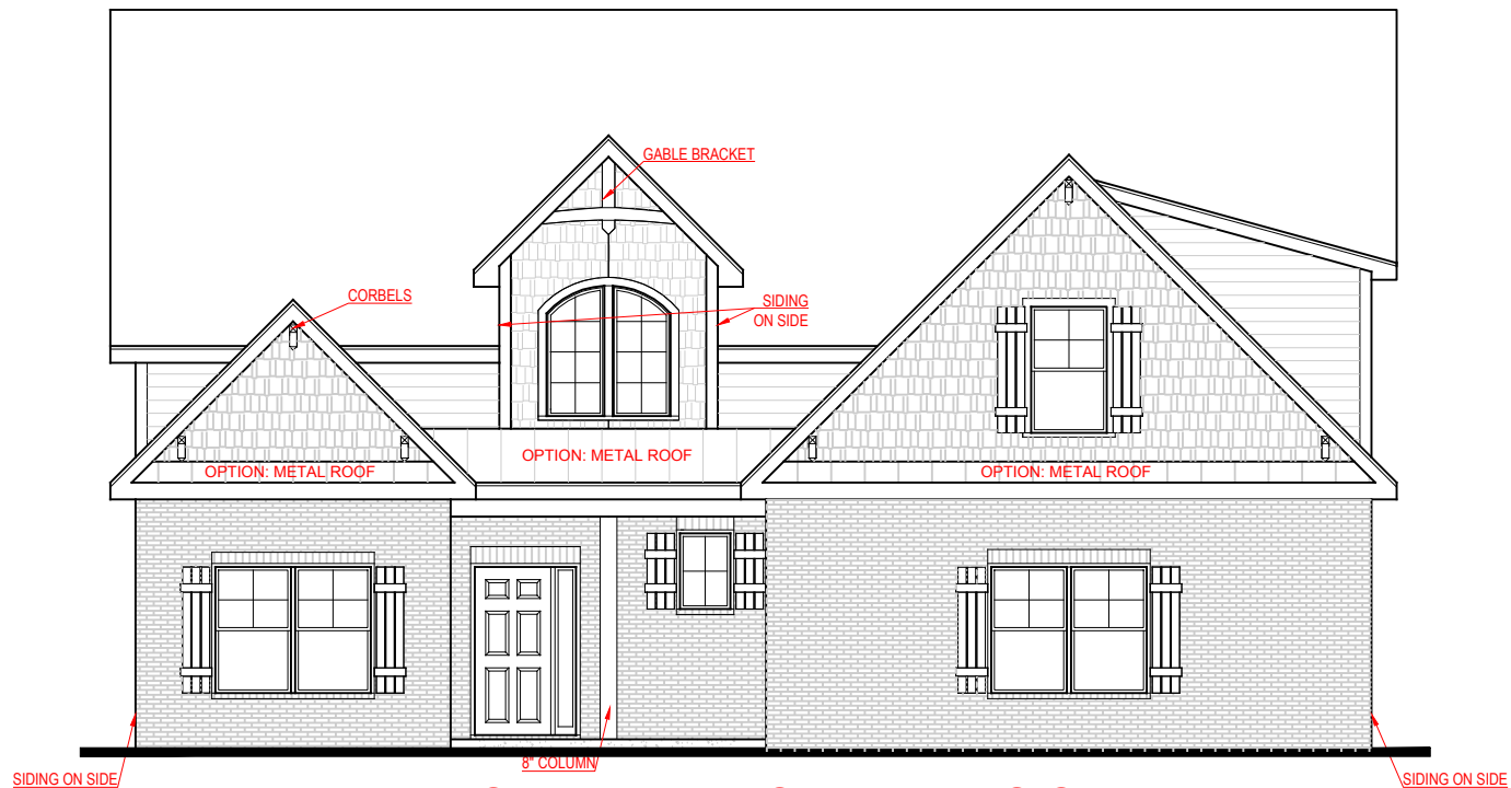
FRONT ELEVATION - D VERSION
