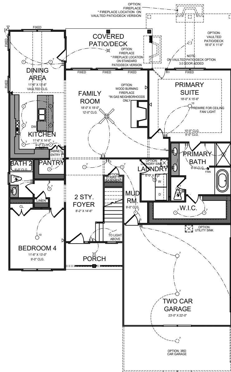
FIRST FLOOR PLAN NO 1ST FLOOR
