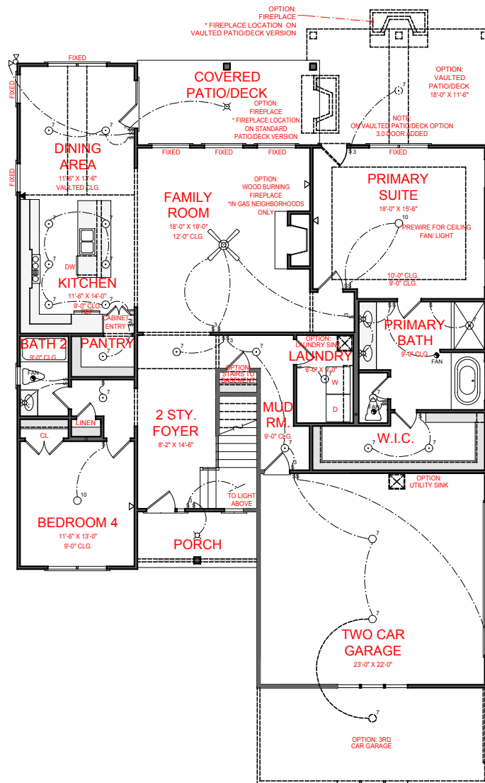
FIRST FLOOR PLAN *NO 1ST FLOOR
